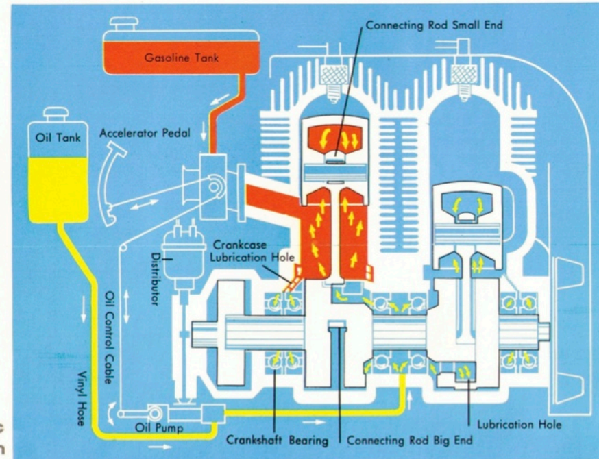
Subarumatic Lubrication Diagram
